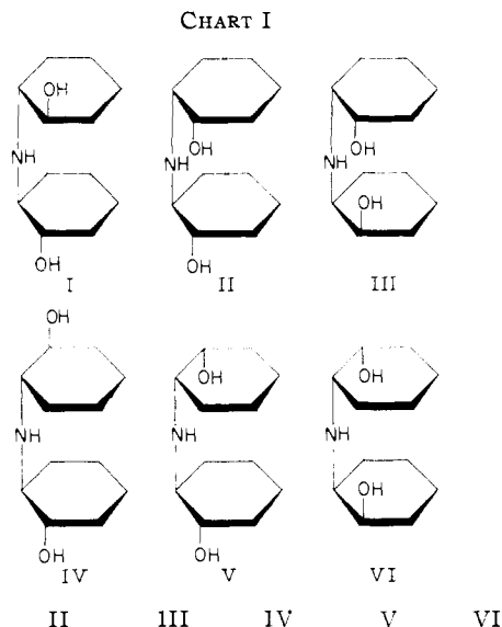
I, meso-trans-trans -2,2'-dihydroxydicyclohexylamine II, dl-trans-cis -2,2'-dihydroxydicyclohexylamine III, meso-cis-cis -2,2'-dihydroxydicyclohexylamine IV, dl-trans-trans -2,2'-dihydroxydicyclohexylamine V, dl-trans-cis -2,2'-dihydroxydicyclohexylamine VI, dl-cis-cis -2,2'-dihydroxydicyclohexylamine
